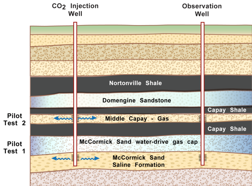
Figure 2. Geologic section at the Rosetta pilot site.
