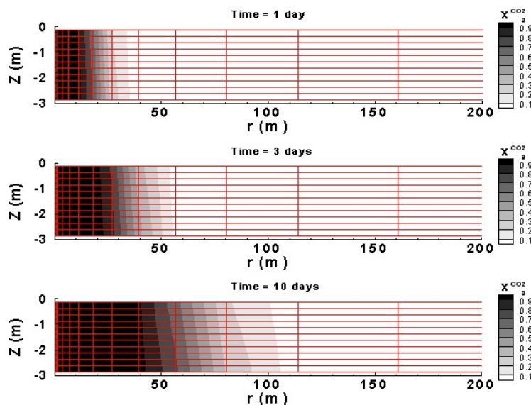
Figure 4. Two-dimensional r - z results showing \text{CO}_2 mass fraction in the gas phase ( X_g^{\text{CO}_2} ) at three times for injection into the gas interval, assuming radial symmetry in the Capay Shale sand stringer.
