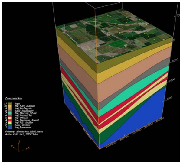
Initial geomodel of WESTCARB Phase III large-volume CO 2 storage test site in San Joaquin Basin below the Kimberlina site
