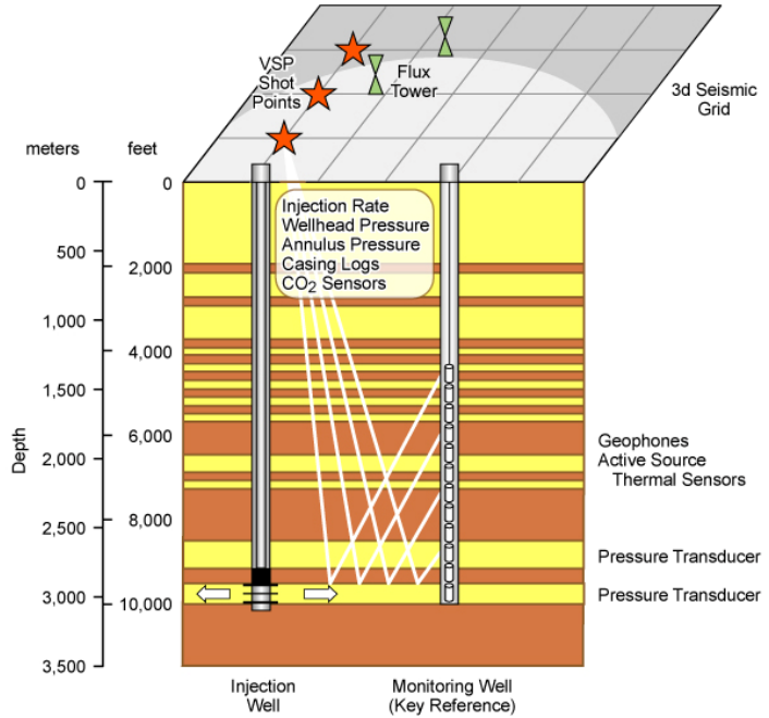
WESTCARB Phase III proposed approach to surface and subsurface monitoring
